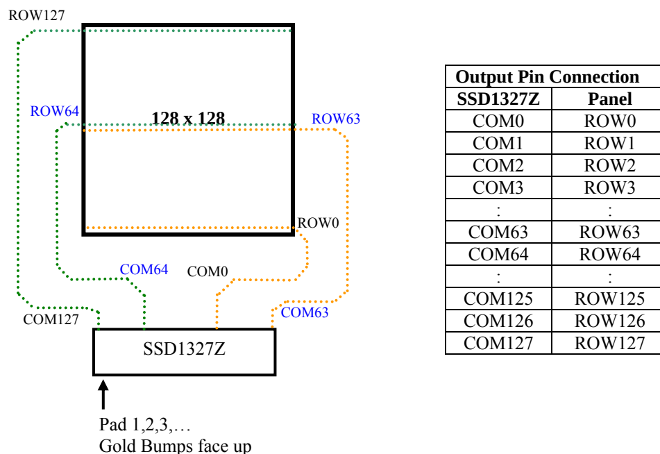
Figure 10-4: Output pin assignment when command A0h bit A[6]=0.
