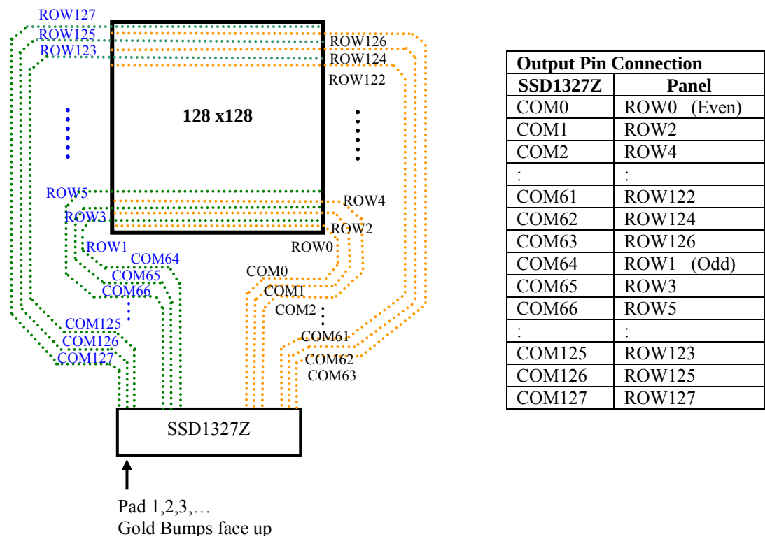
Figure 10-5 : Output pin assignment when command A0h bit A[6]=1.
