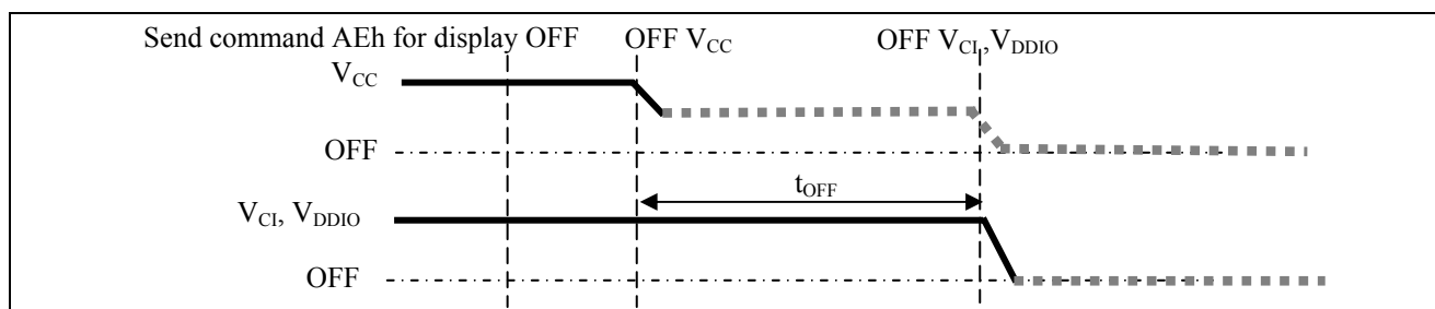
Figure 8-14 : The Power OFF sequence
