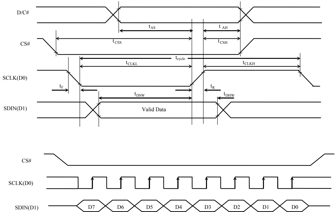
Figure 13-3 : Serial interface characteristics (4-wire SPI)
