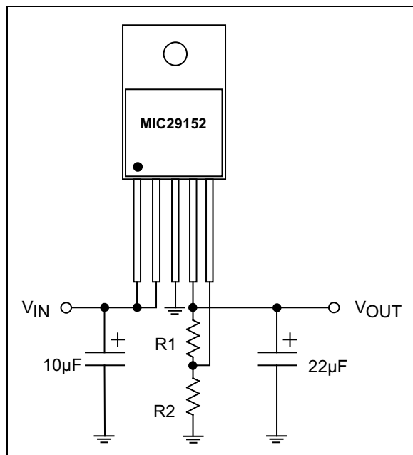
FIGURE 4-2: Adjustable Regulator with Resistors.
