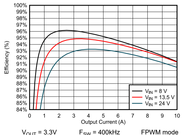
Figure 8-6. Efficiency
