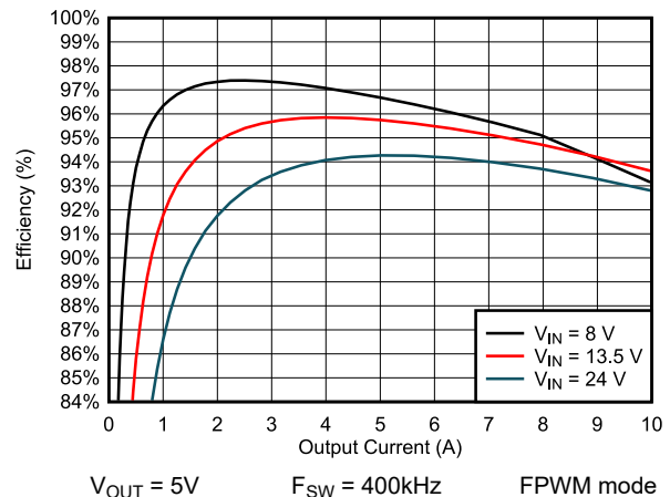
Figure 8-4. Efficiency
