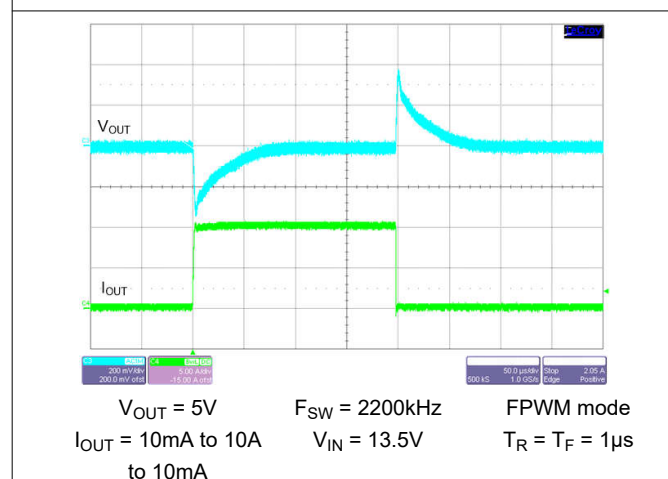
Figure 8-41. Load Transient
