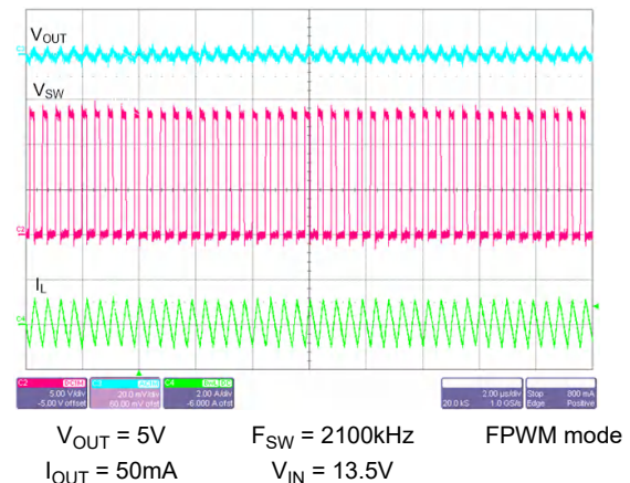
Figure 8-28. Switching Waveform and V_{OUT} Ripple
