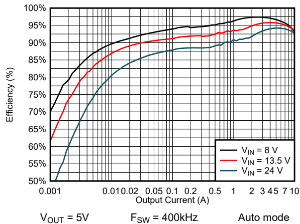
Figure 8-3. Efficiency
