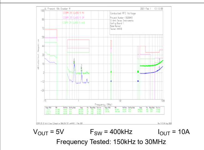
Figure 8-44. Conducted EMI versus CISPR25 Class 5 Limits (Green: Peak Signal, Blue: Average Signal)
