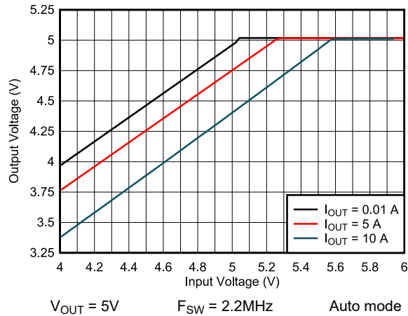
Figure 8-21. Dropout
