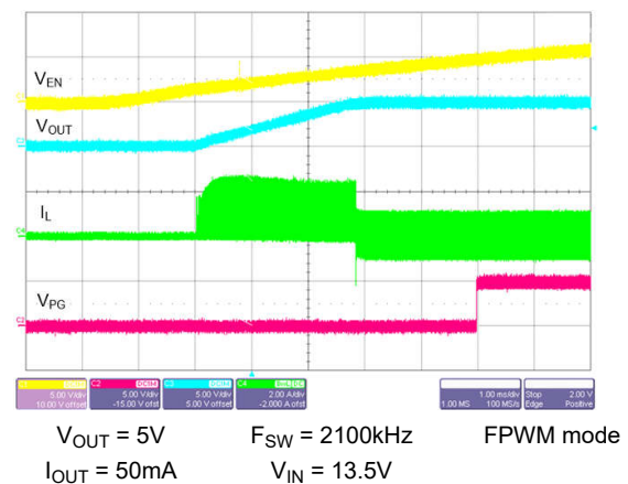
Figure 8-30. Start-Up With 50mA Load
