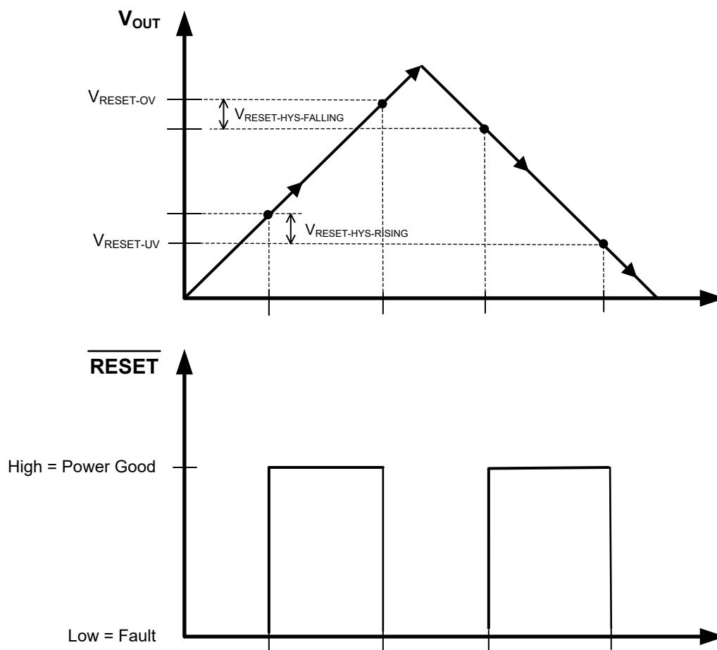
Figure 7-7. \overline{\text{RESET}} Static Voltage Thresholds
