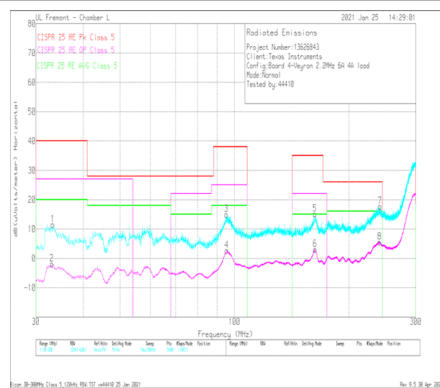
Figure 8-51. Radiated EMI Bicon Horizontal vs CISPR25 Class 5 Limits
