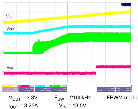
Figure 8-31. Start-Up With 3.25A Load
