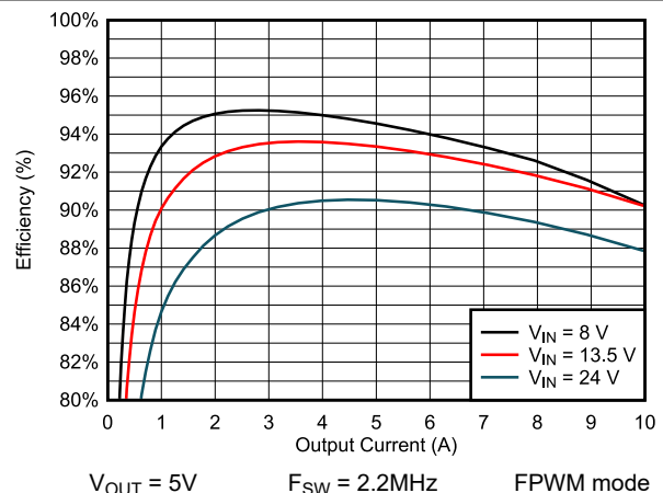
Figure 8-8. Efficiency
