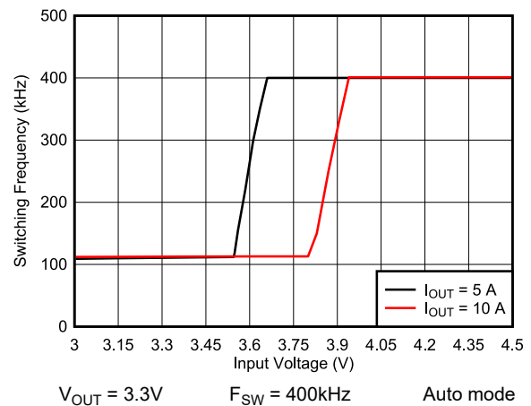
Figure 8-24. Frequency Dropout
