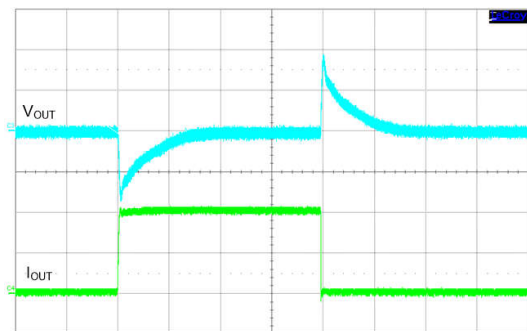
Figure 8-36. Load Transient
