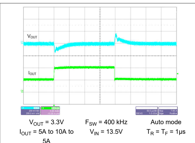
Figure 8-40. Load Transient
