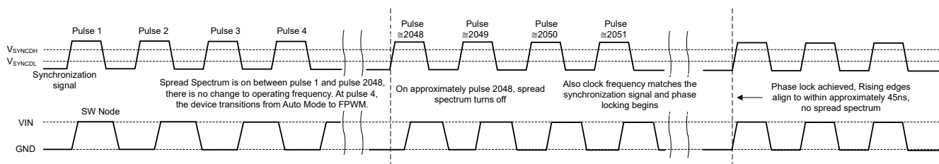
Figure 7-5. Synchronization Process
