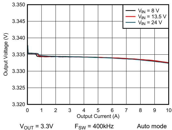
Figure 8-13. Load and Line Regulation
