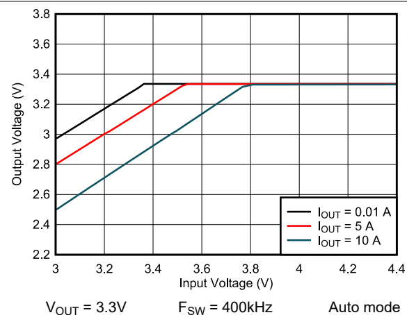
Figure 8-20. Dropout
