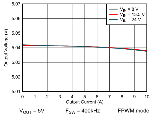
Figure 8-12. Load and Line Regulation
