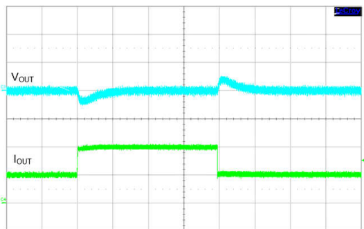
Figure 8-35. Load Transient
