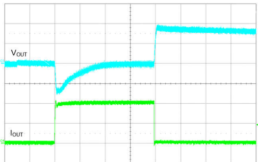
Figure 8-33. Short-Circuit Recovery
