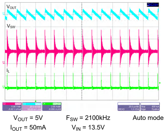
Figure 8-27. Switching Waveform and V_{OUT} Ripple
