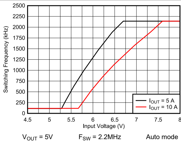
Figure 8-25. Frequency Dropout
