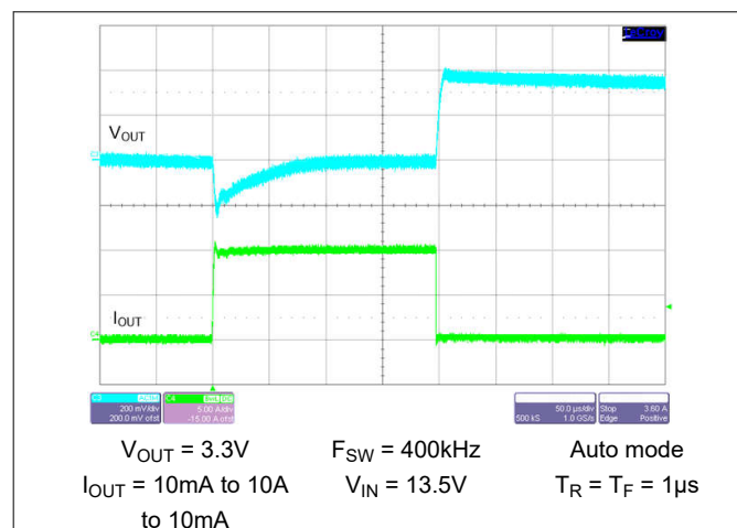
Figure 8-39. Load Transient
