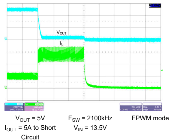
Figure 8-32. Short-Circuit Protection
