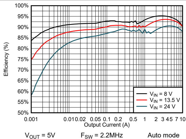
Figure 8-7. Efficiency
