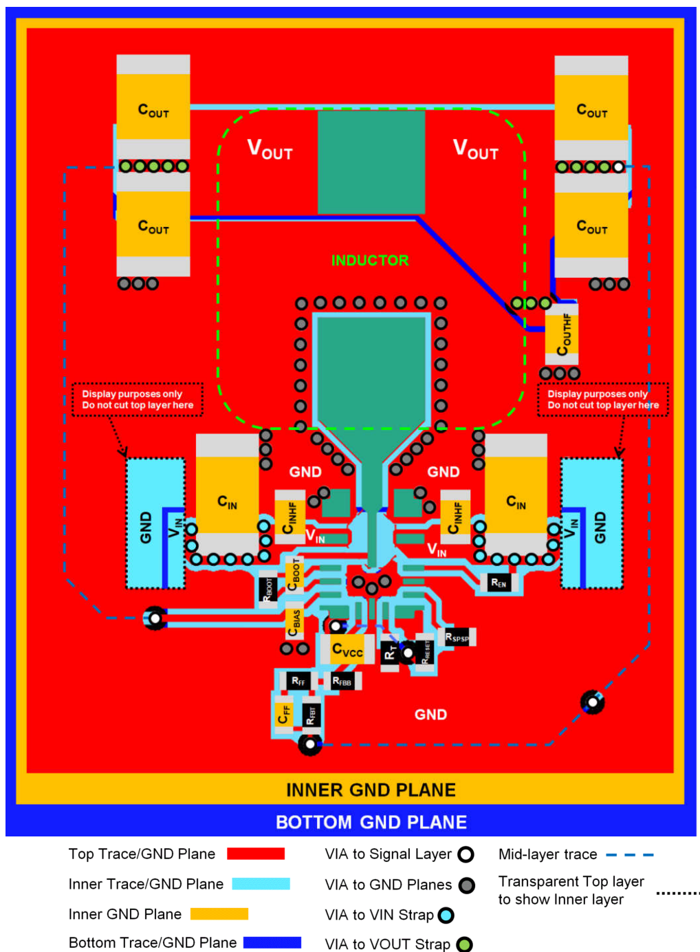
Figure 8-57. Layout Example
