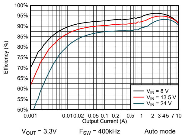
Figure 8-5. Efficiency
