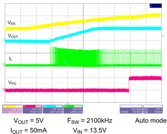
Figure 8-29. Start-Up With 50mA Load
