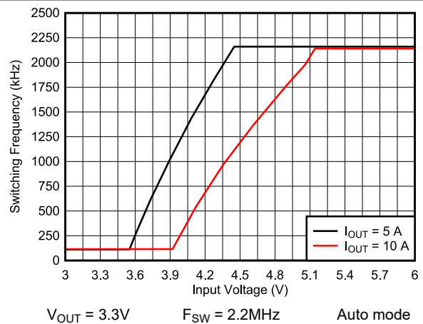
Figure 8-26. Frequency Dropout
