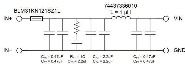
Figure 8-55. Recommended Input EMI Filter
