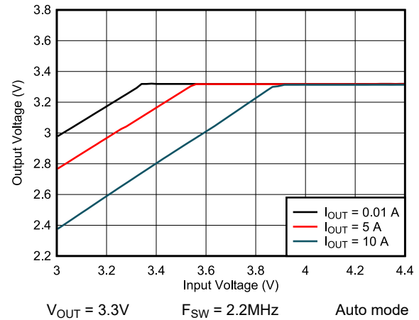
Figure 8-22. Dropout
