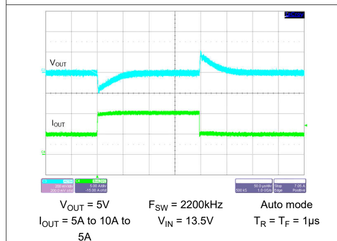
Figure 8-43. Load Transient
