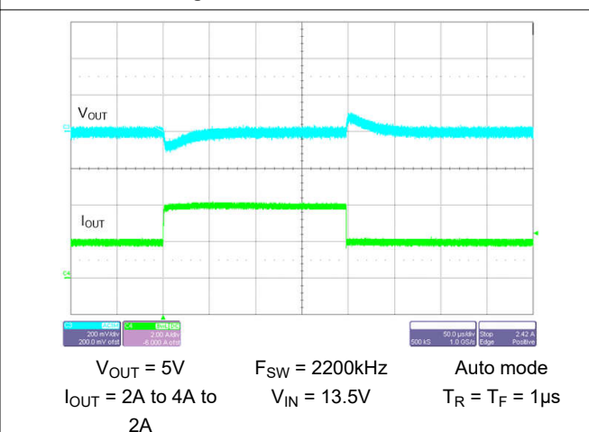
Figure 8-42. Load Transient
