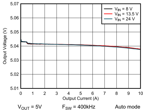
Figure 8-11. Load and Line Regulation
