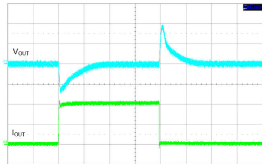
Figure 8-34. Recovery from Dropout
