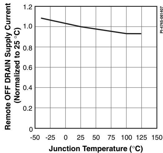
Figure 52. Remote-OFF DRAIN Supply Current vs. Temperature.
