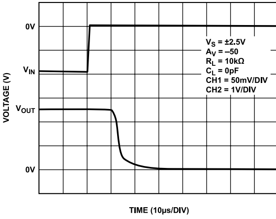
Figure 28. Negative Overvoltage Recovery
