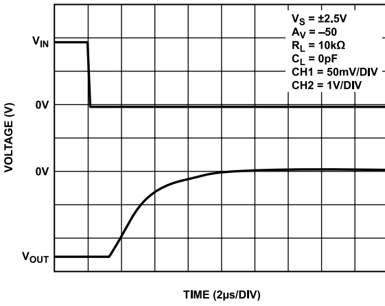
Figure 27. Positive Overvoltage Recovery
