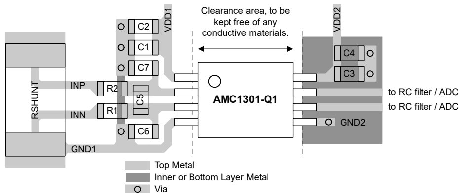
Figure 8-6. Recommended Layout of the AMC1301-Q1
