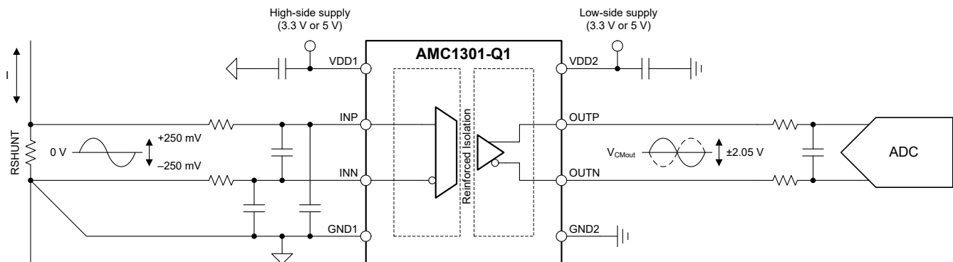
Typical Application
