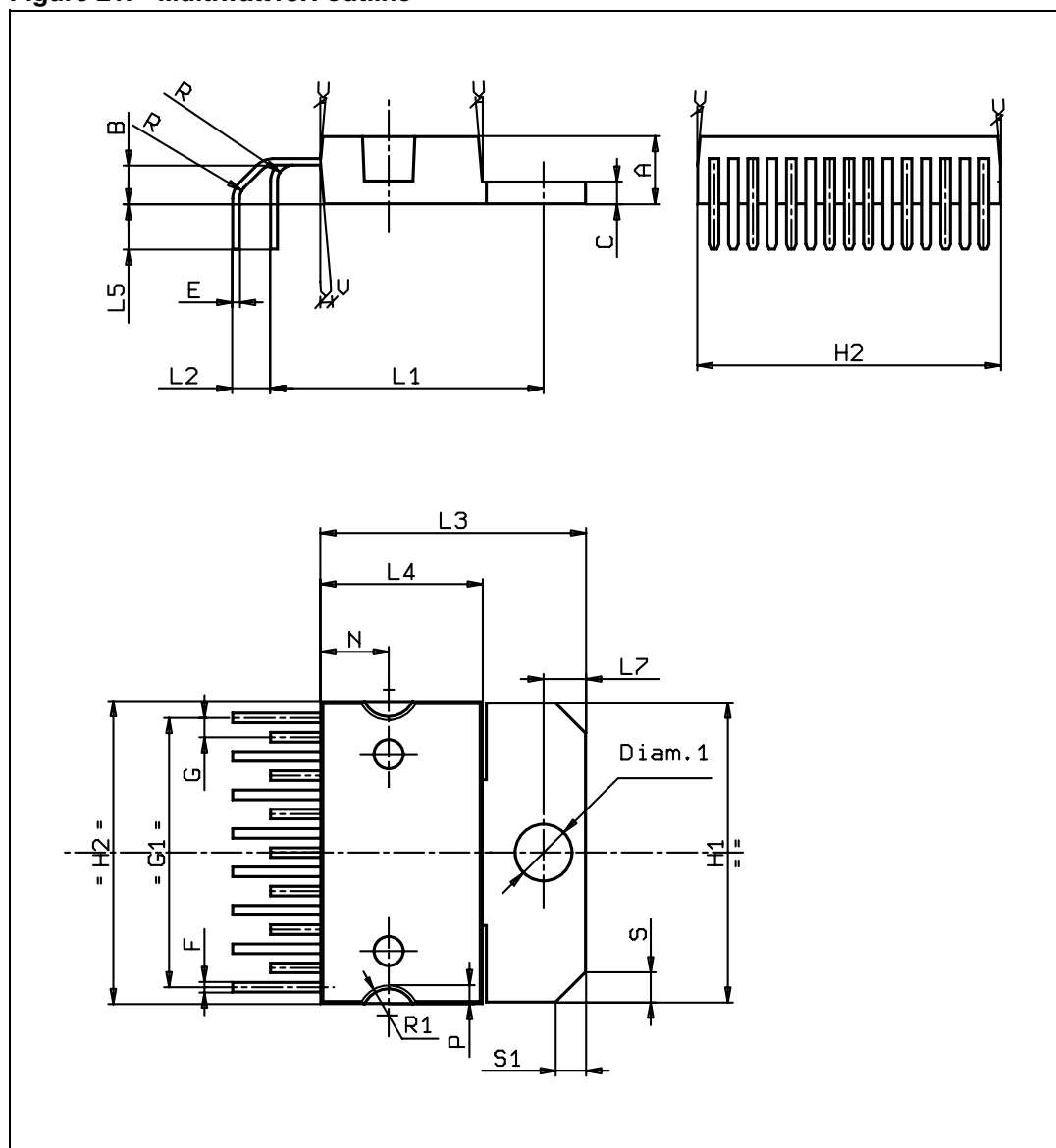
Figure 21. Multiwatt15H outline
