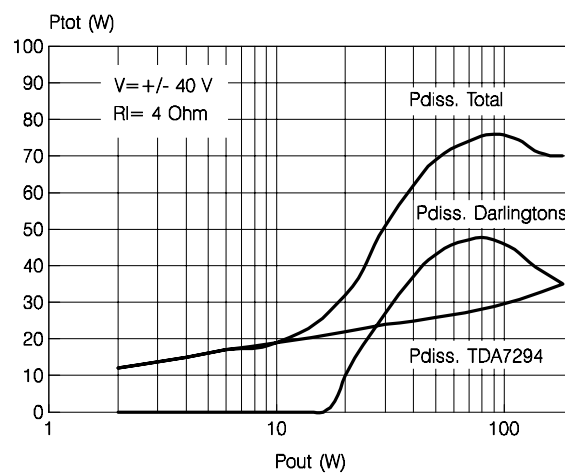
Figure 25. Power dissipation vs. output power (RI = 4 Ω)
