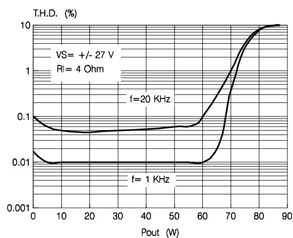
Figure 8. Distortion vs. output power ( R_L = 4 \Omega )
