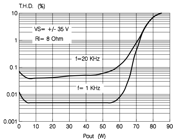
Figure 6. Distortion vs. output power ( R_L = 8 \Omega )
