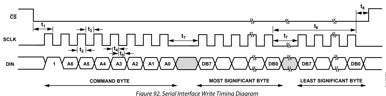
Figure 92. Serial Interface Write Timing Diagram
