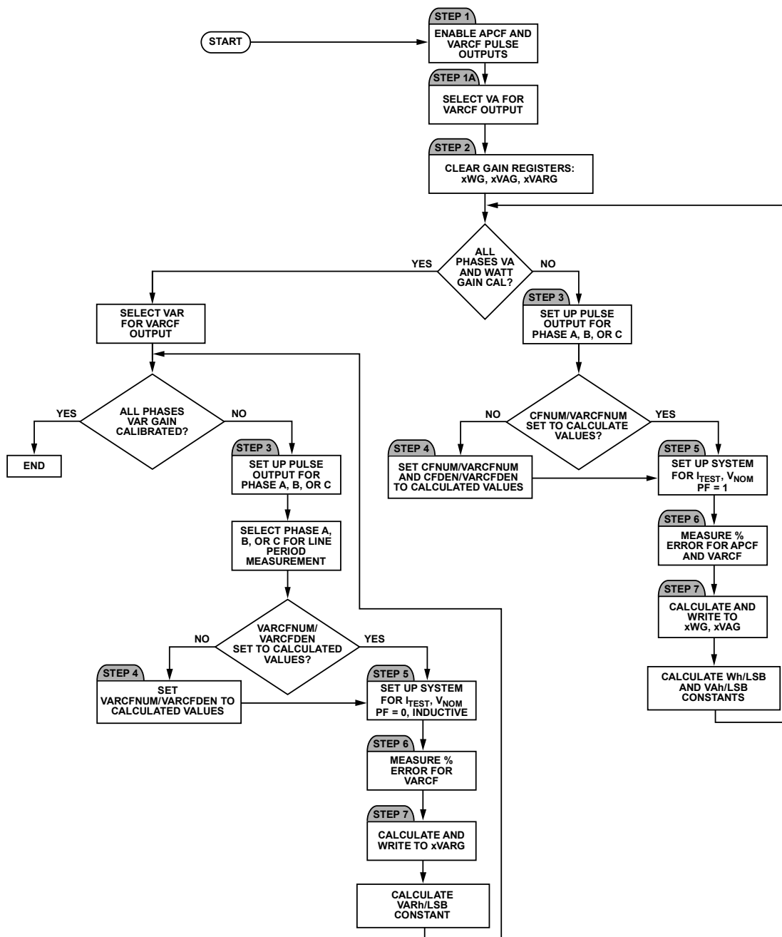
Figure 78. Gain Calibration Using Pulse Output
