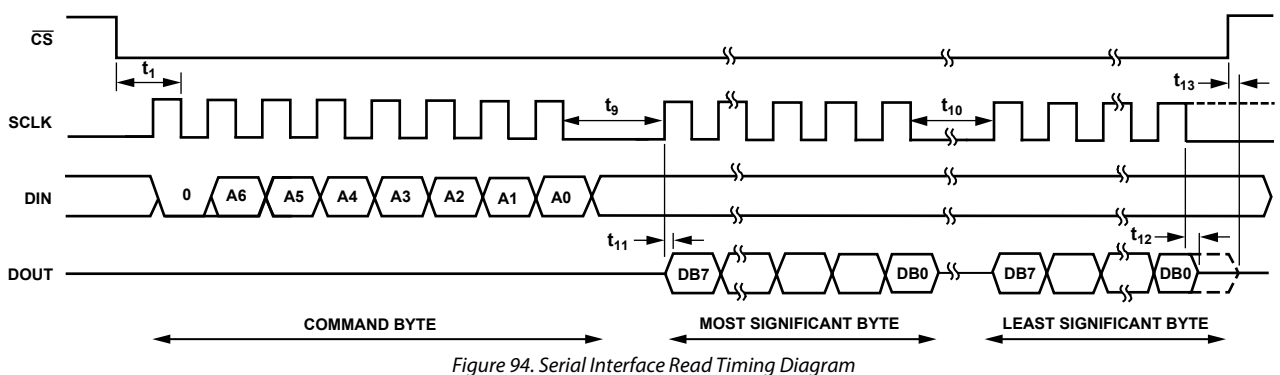
Figure 94. Serial Interface Read Timing Diagram
