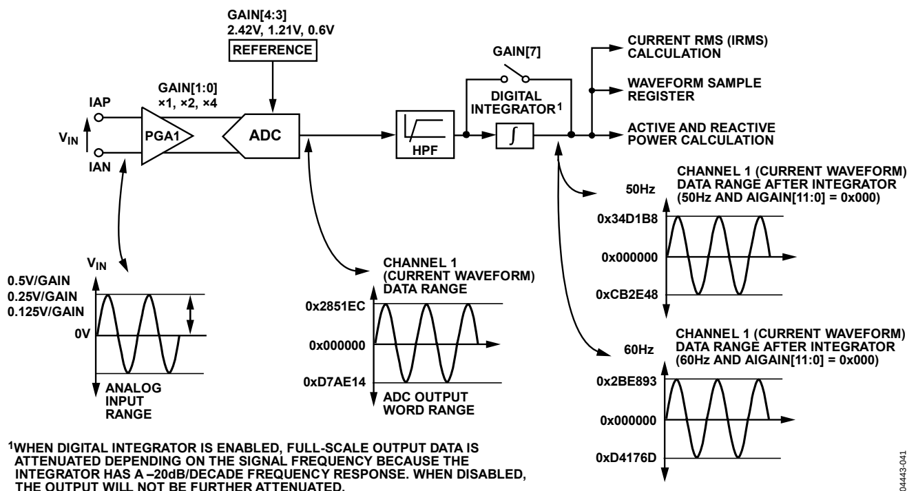
Figure 41. Current Channel Signal Path
