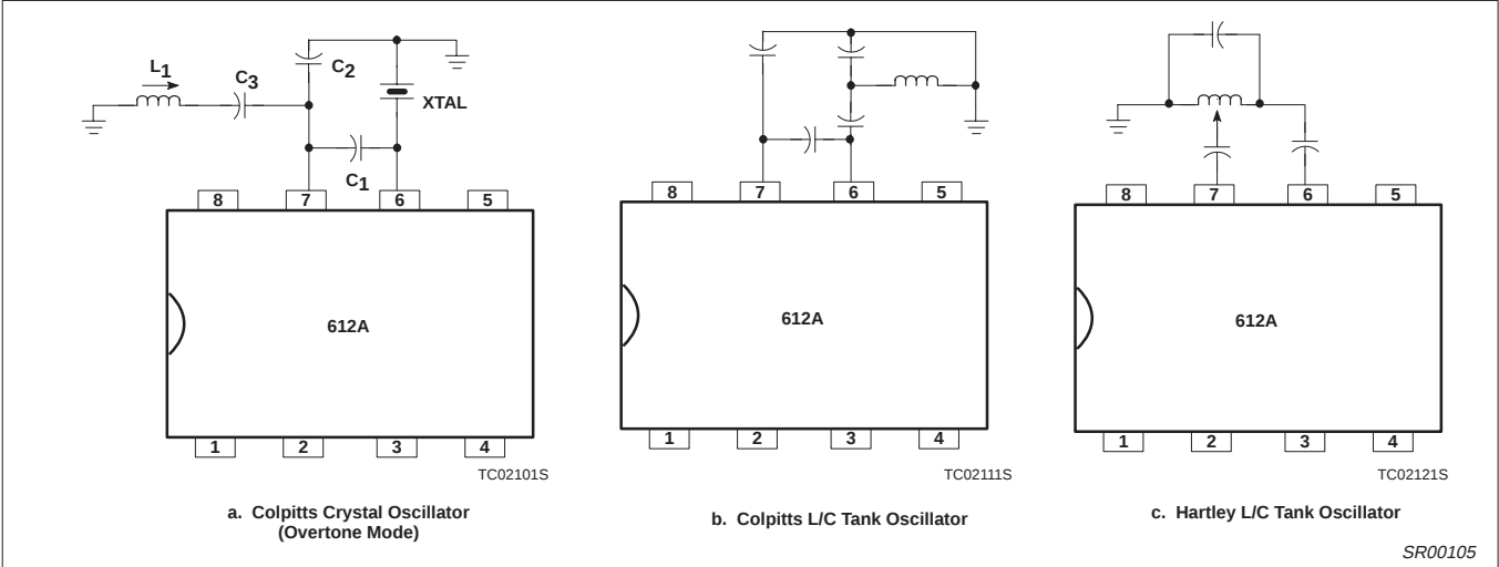
Figure 7. Oscillator Circuits
