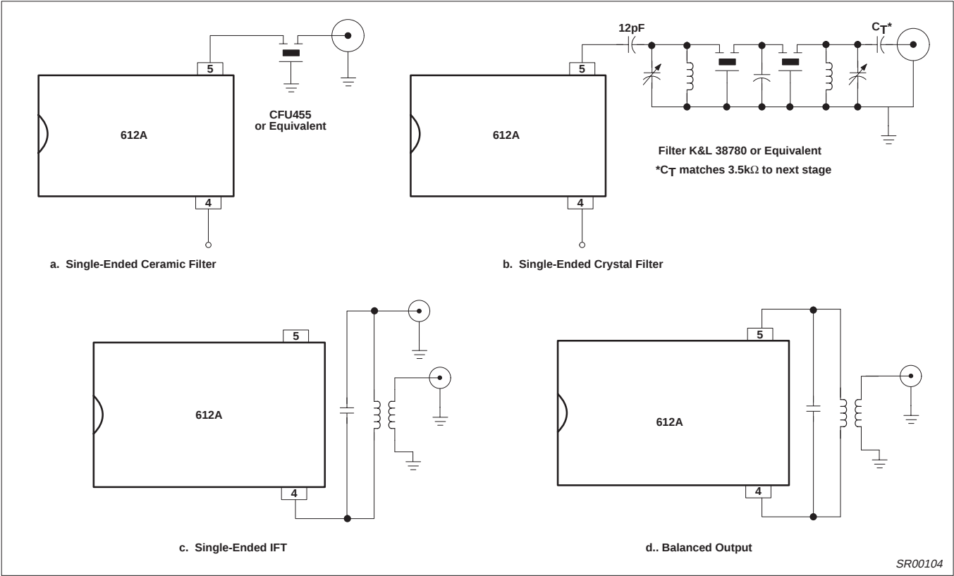
Figure 6. Output Configuration
