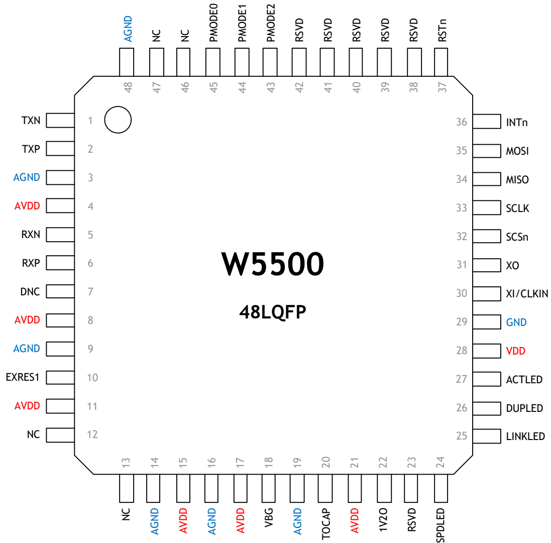
Figure 1. W5500 Pin Layout
