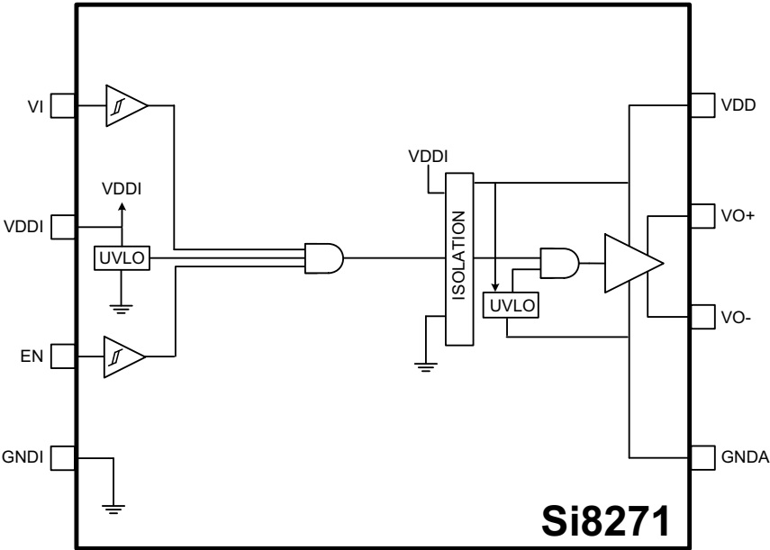
Figure 4. Si8271 Block Diagram
