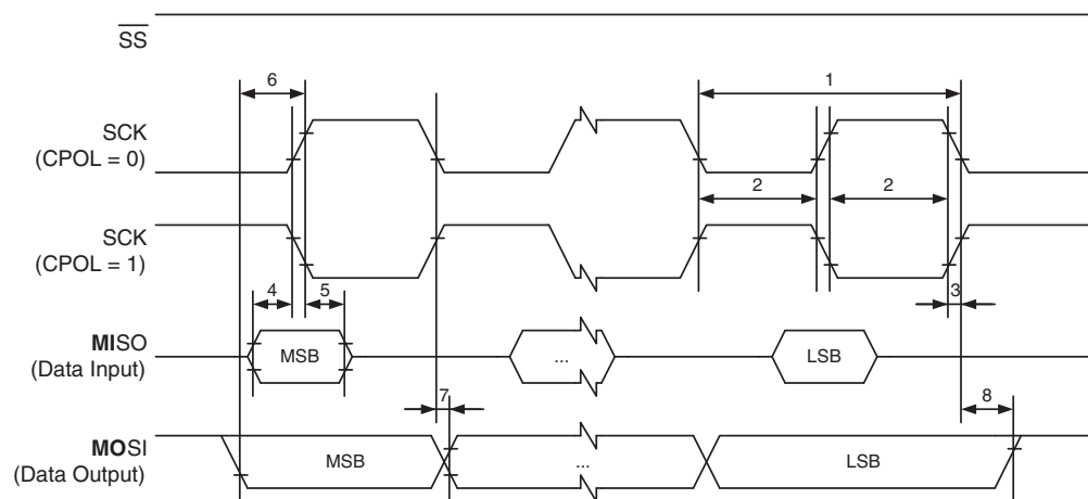
Figure 31-7. SPI Interface Timing Requirements (Master Mode)
