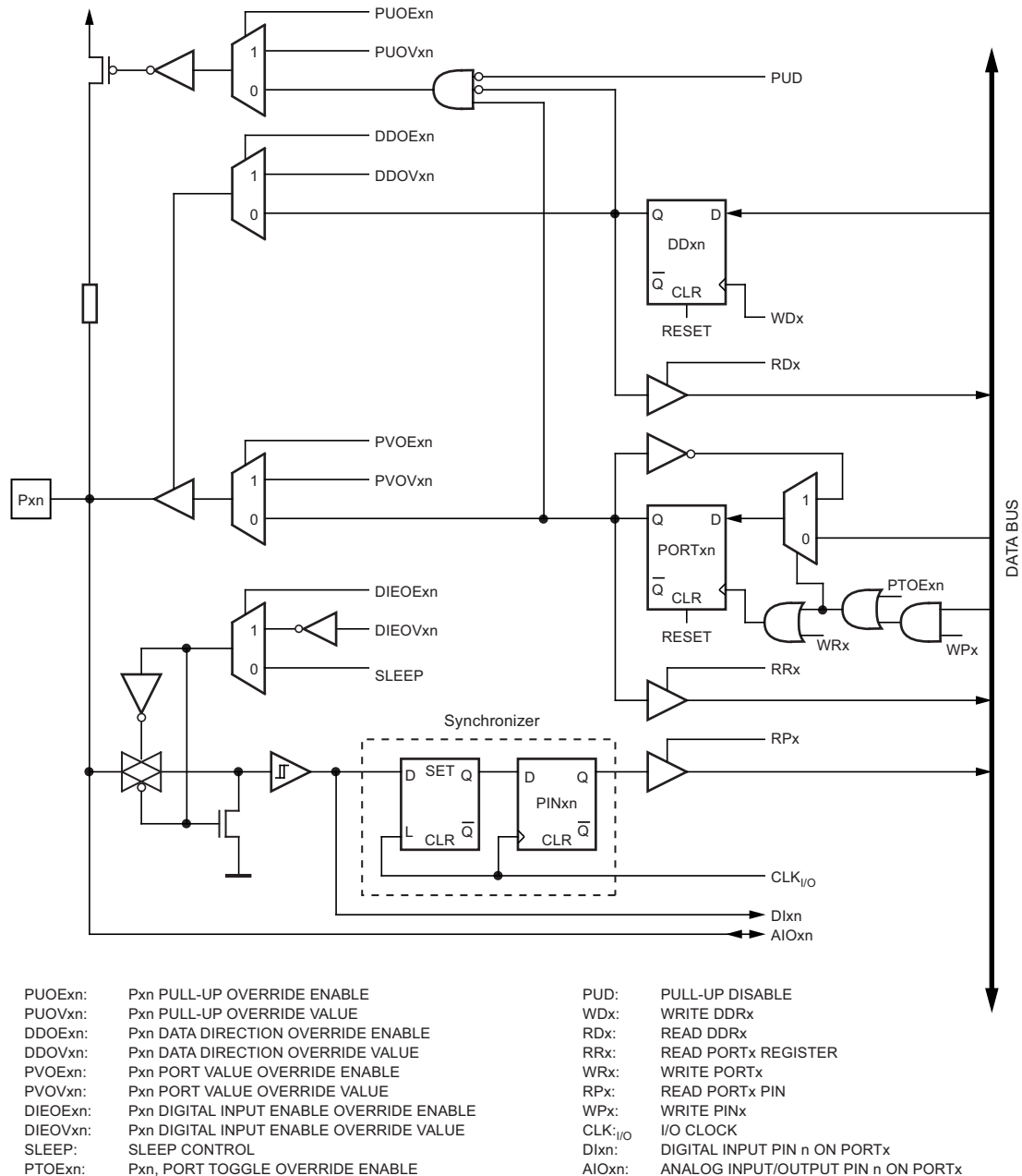
Figure 13-5. Alternate Port Functions (1)
