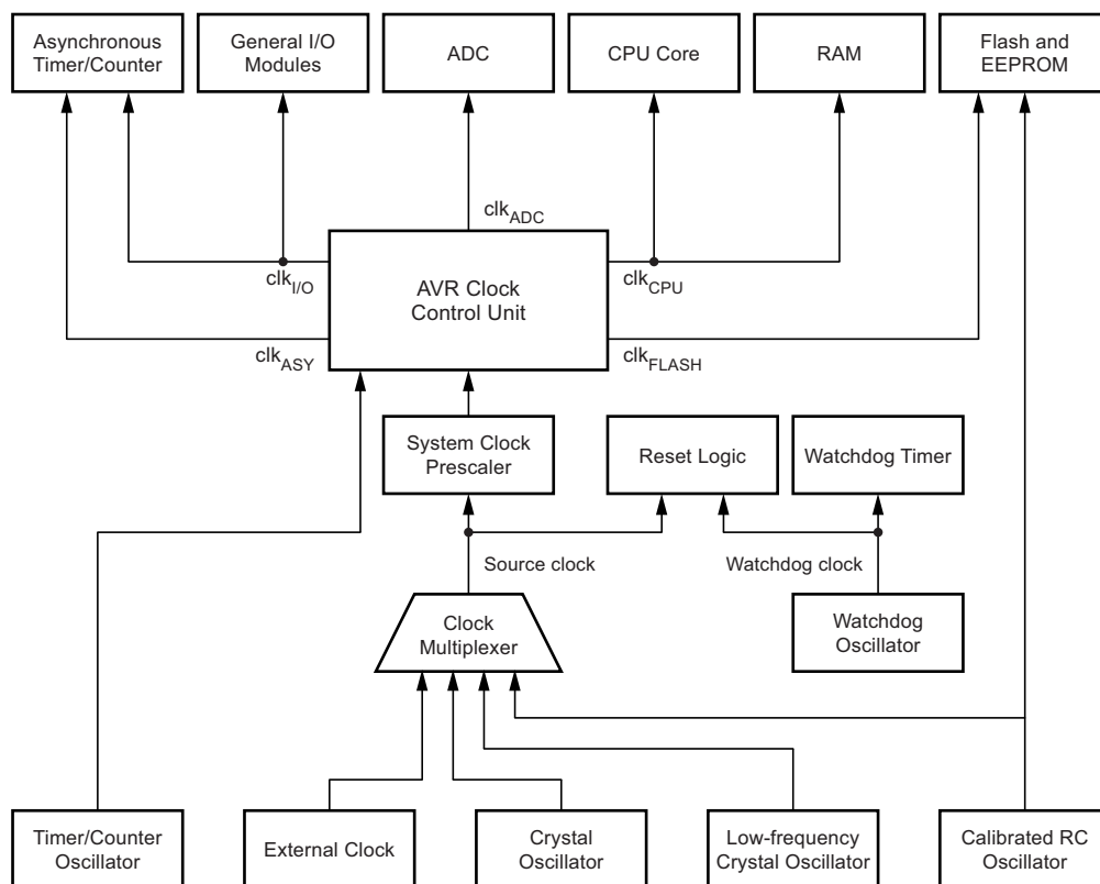
Figure 8-1. Clock Distribution
