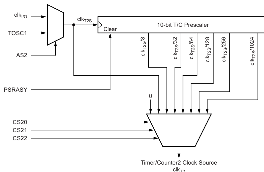
Figure 17-12.Prescaler for Timer/Counter2
