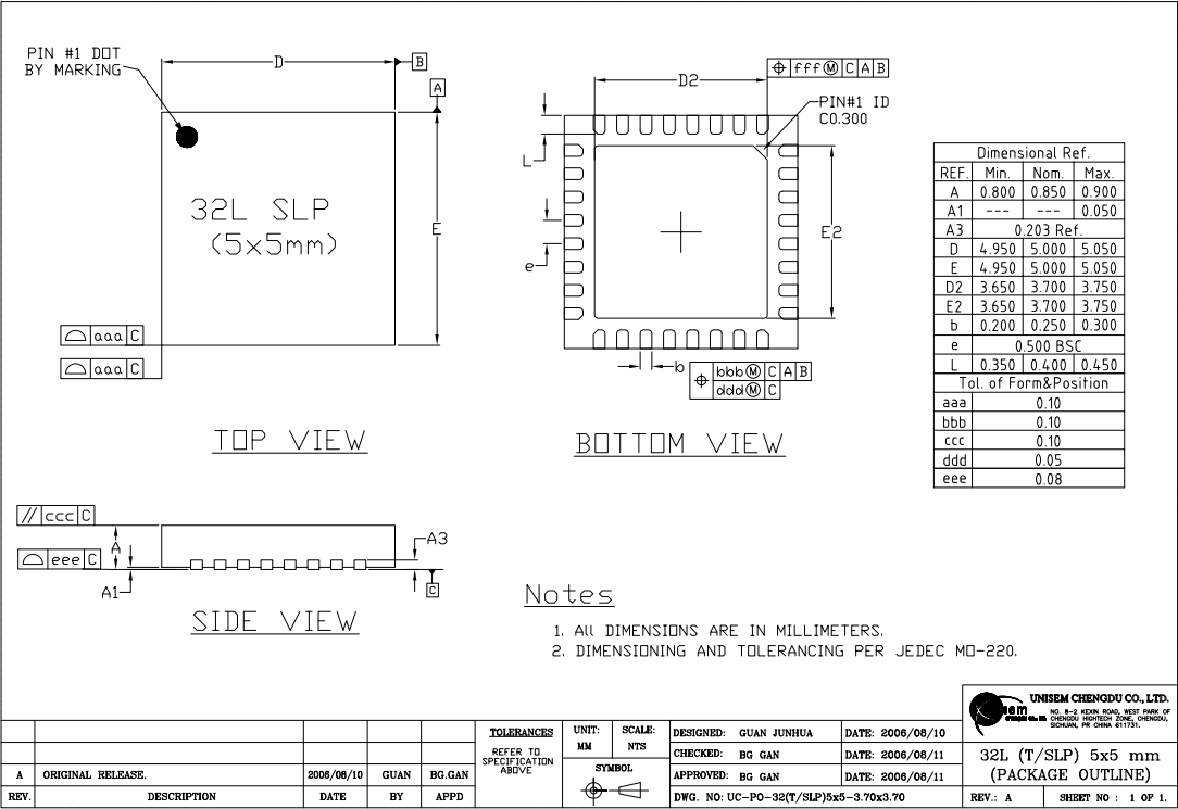
Figure 6-1. ESP8266EX Package
