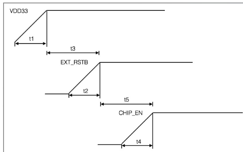
Figure 5-1. ESP8266EX Power-up and Reset Timing
