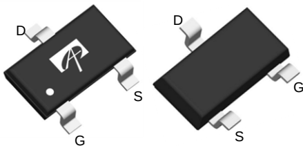
SOT23 Top View Bottom View
