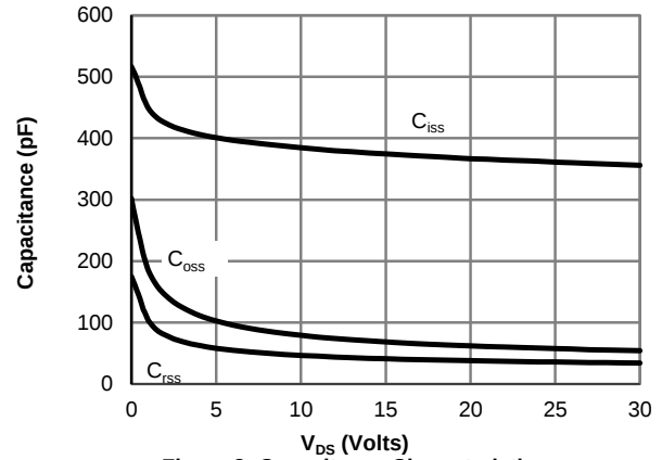
Figure 8: Capacitance Characteristics
